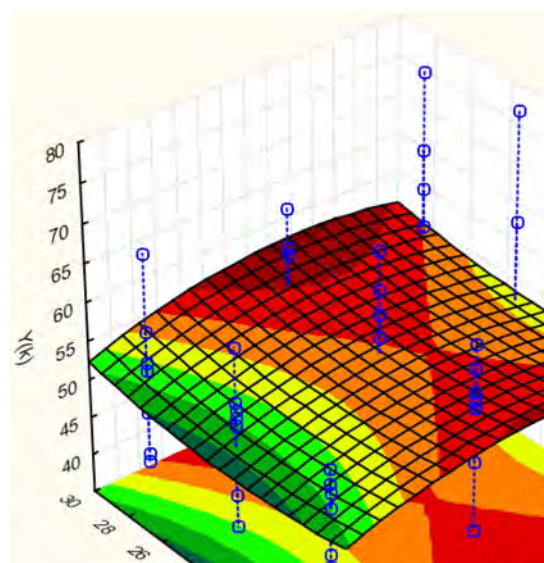
Y = f(x_1x_5)
