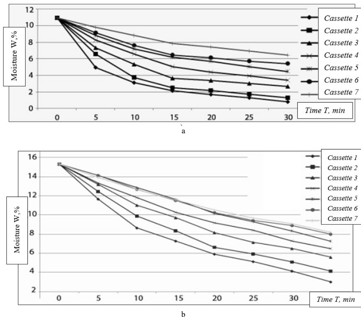
Figure 4 – Change in seed moisture content during drying in a pilot plant (a) with an initial humidity of 11% and a drying agent temperature of 60–65°C and (b) with an initial humidity of 15.5% and a drying agent temperature of 45–50°C
